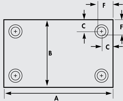
Four Post - Type 4P
