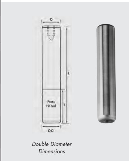
Double Diameter Pin Dimensions
